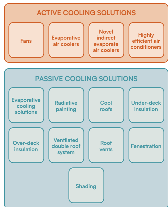
Figure 1. Diagram of mapped space cooling solutions
