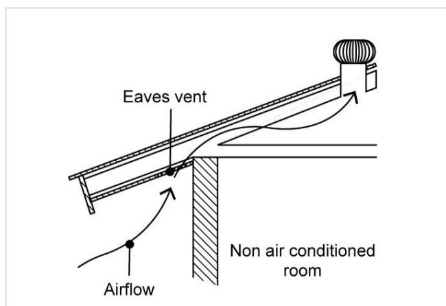
Figure 16. Diagram on use of roof vents and importance of airflow in the eaves vent. Source: Adapted from Yourhome — Australia's guide to environmentally sustainable homes.
