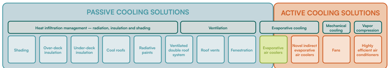
Figure 3. Diagram of mapped space cooling solutions in this report. Own elaboration based on SELCO Foundation’s Access to Sustainable Cooling report .
