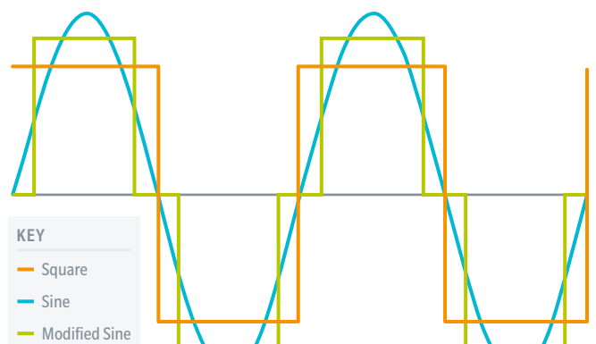
Figure 3 – Inverter waveforms
