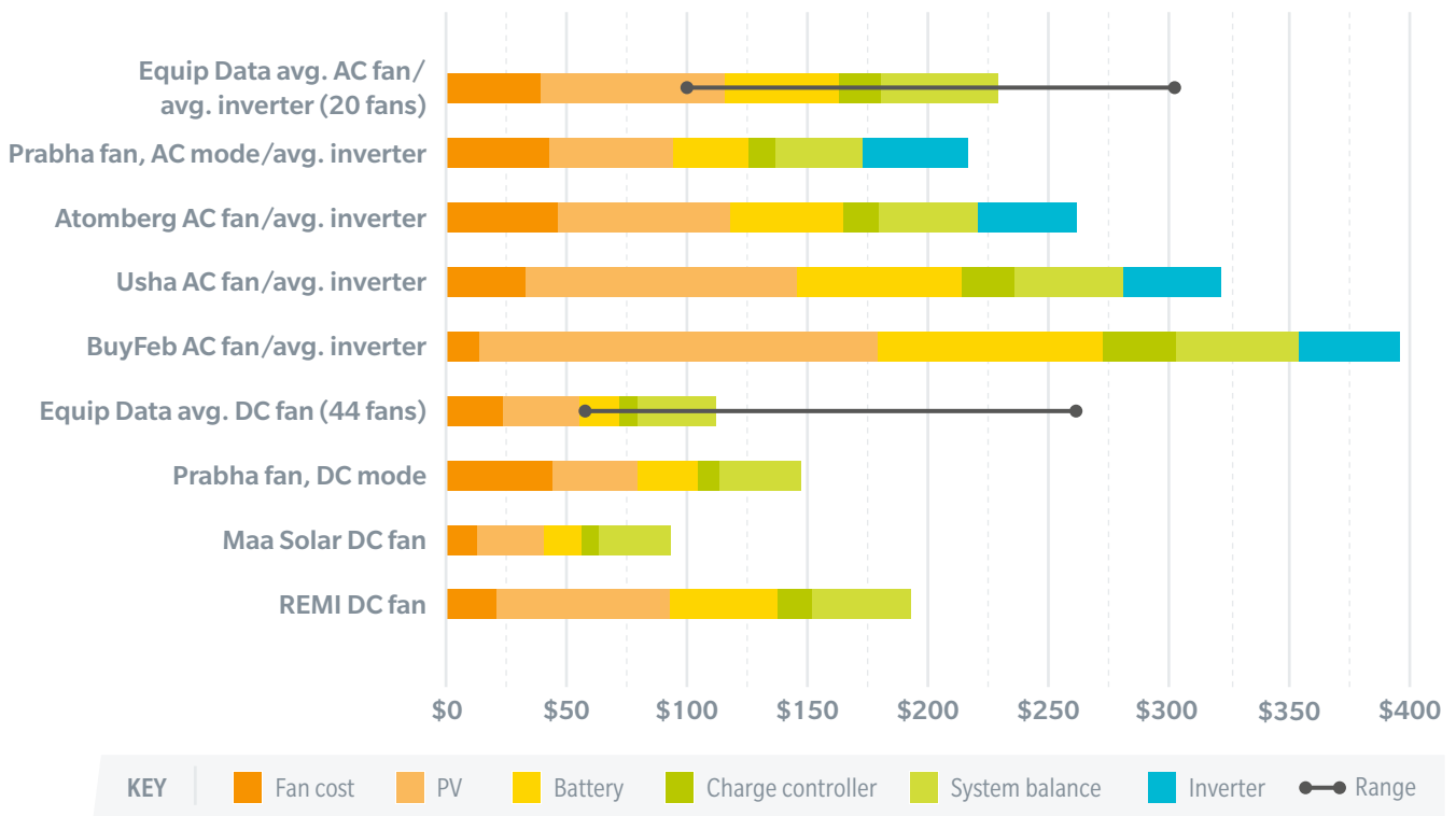
Figure 29 – Total system cost for AC pedestal and table fans with inverters, compared to DC fans, and average of AC and DC fans from Equip Data
