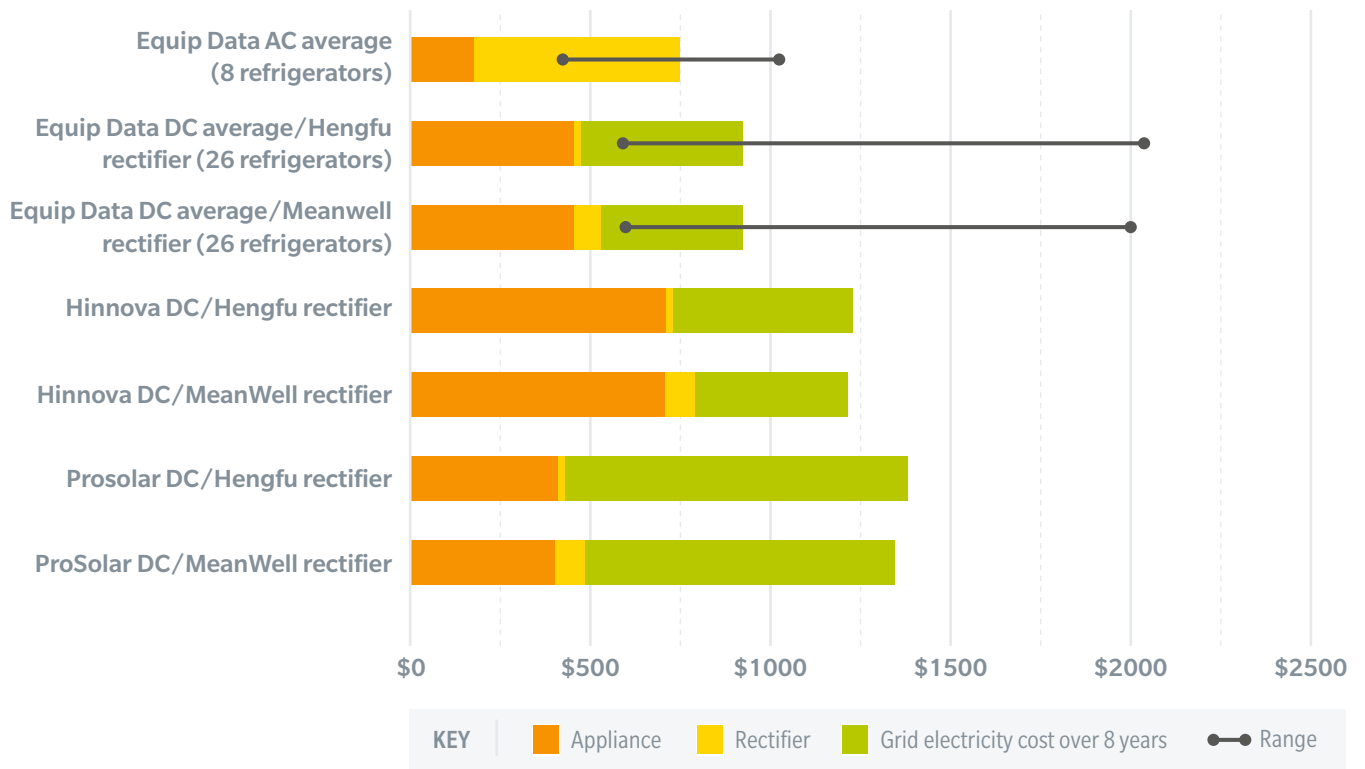
Figure 21 – Simple lifecycle cost of the tested DC refrigerators with rectifiers running on an AC mini-grid, and comparison with average AC and DC models from Equip Data
