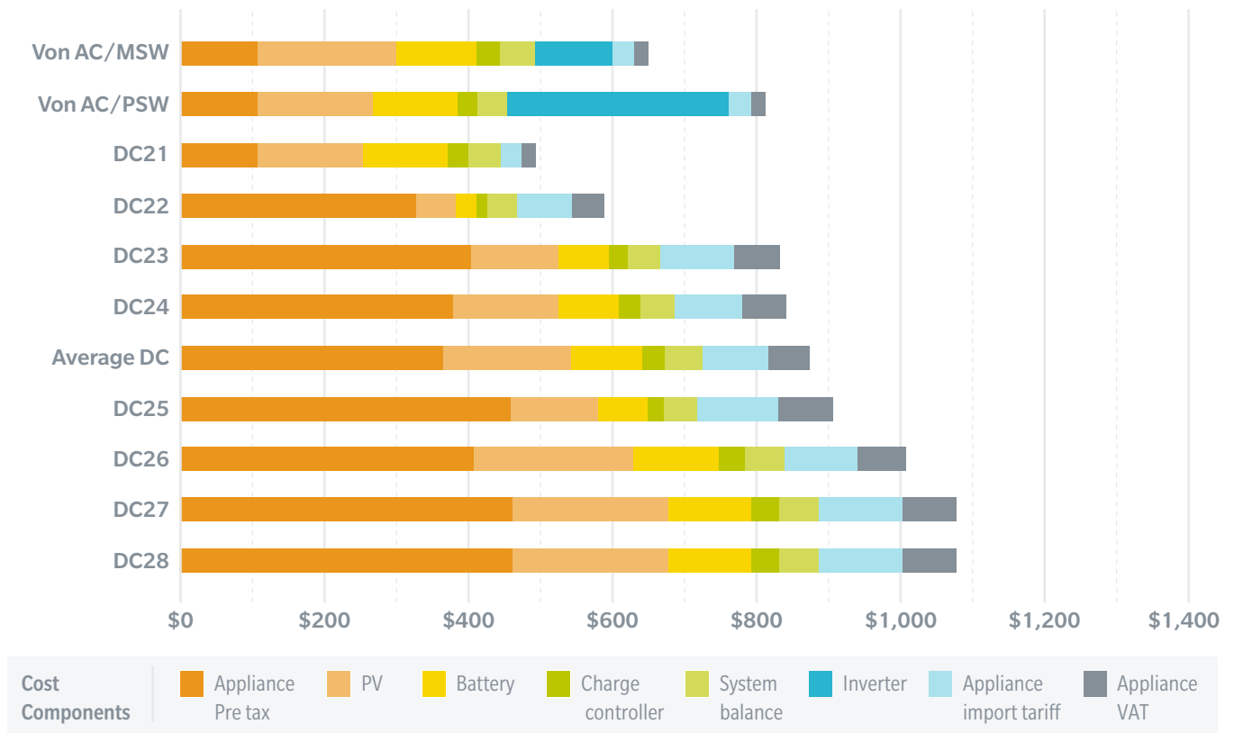
Figure 32– Total system cost of Von AC refrigerator with MSW and PSW inverters compared to the average of similarly sized DC refrigerators in native mode (capacity 90-120 litres), inclusive of VAT and import duty
