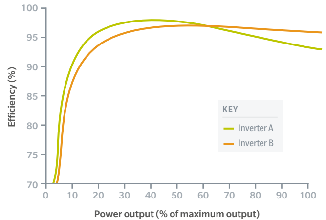
Figure 2a – Example of inverter efficiency curves 6
