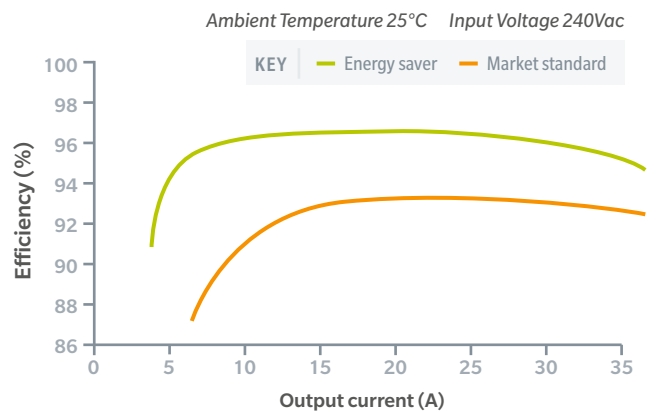
Figure 2b – Example of rectifier efficiency curves 7
